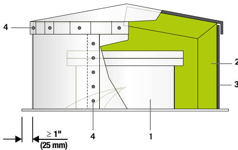
1. Manhole - 2. ProRox insulation - 3. Cladding (jacketing) - 4. Sheet-metal screw
