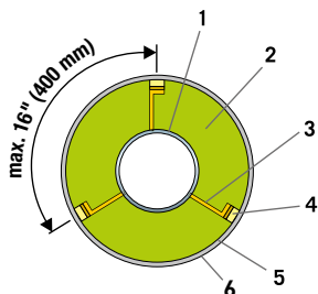
1. Pipe - 2. ProRox insulation - 3. Spacer - 4. Thermal dividing layer - 5. Support ring - 6. Cladding (jacketing)
