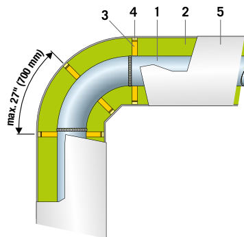
1. Pipe - 2. ProRox insulation - 3. Spacer - 4. Thermal dividing layer - 5. Cladding (jacketing)
