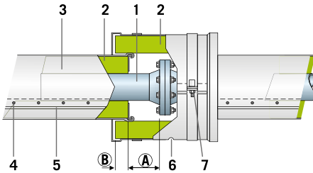
1. Pipe - 2. ProRox insulation - 3. Cladding (jacketing) - 4. Sheet-metal screw or rivet - 5. Swage - 6. Drainage opening - 7. Straps - \textcircled{B} \geq 2" (50 mm) - \textcircled{A} = \text{Bolt length} + 1.2" (30 mm)
